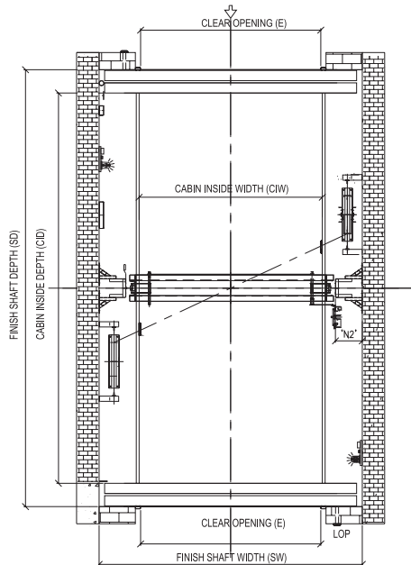
Same Side Ent Floor PLAN OF LIFT SHAFT
