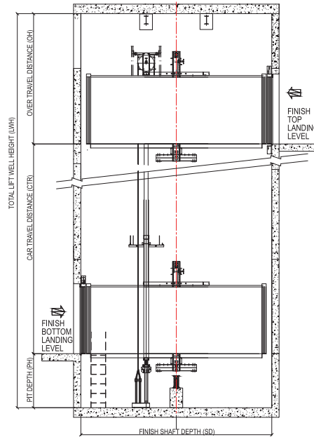
SECTION 'X-X' SHAFT ELEVATION
