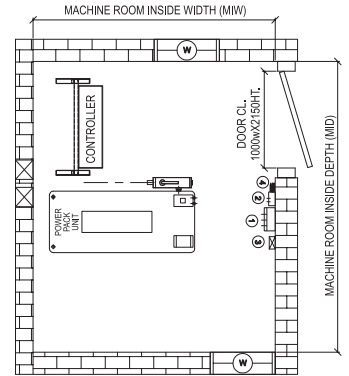
MACHINE ROOM VIEW
