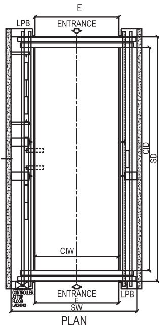
PLAN
