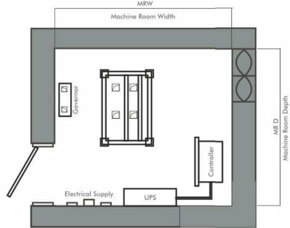
Machine Room Plan Layout
